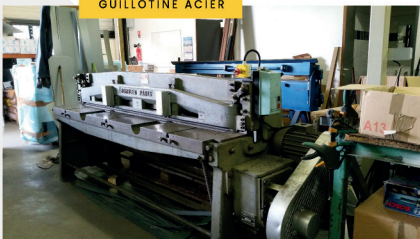
GUILLOTINE ACIER
