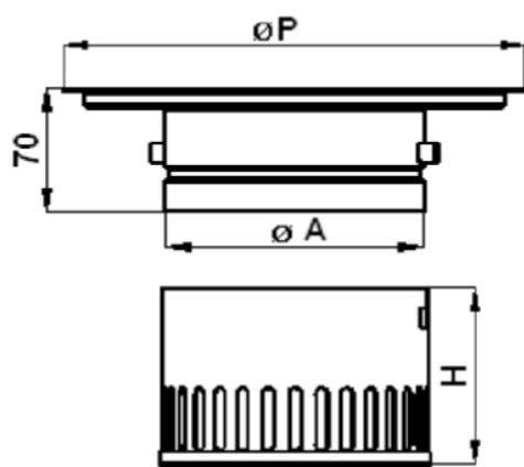
Dimensions KDP
