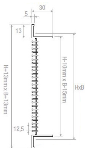
GRILLE KBL20-S
