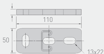
Dimensions PS641
