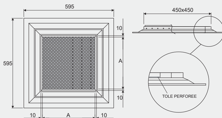
Dimensions KH2-SR
