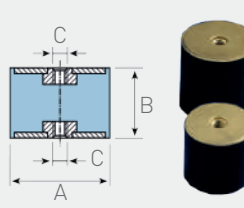
Plot cylindrique Type C
